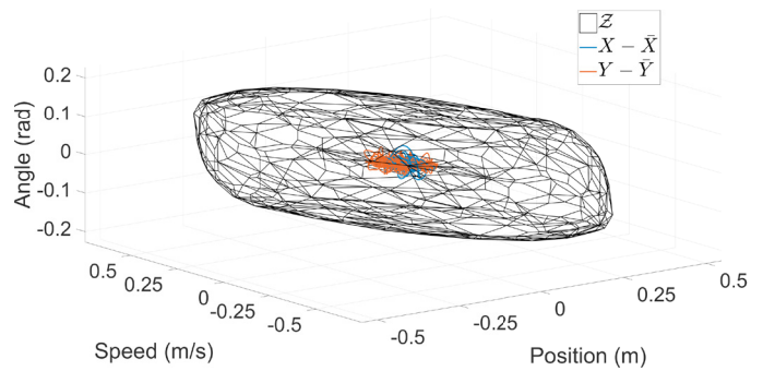
Fig. 2. Invariant set \mathcal{Z} and the trajectory of the system error for the directions x and y during the validation flight in the state-space position-speed-angle.
