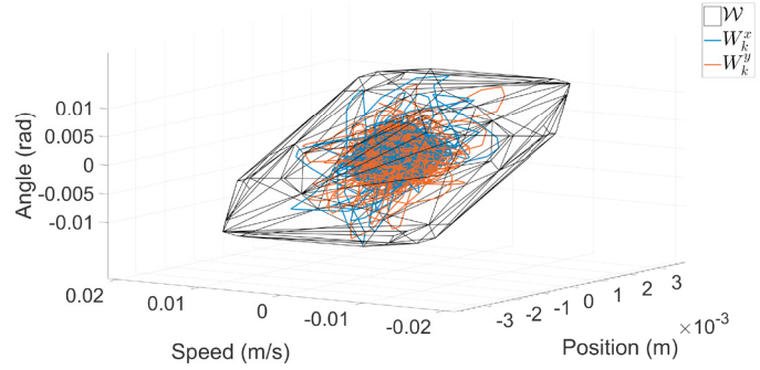
Fig. 1. Disturbance set \mathcal{W} identified and further used for the TB MPC design, and disturbance realizations during the validation flight regarding both directions x and y in the state-space position-speed-angle.
