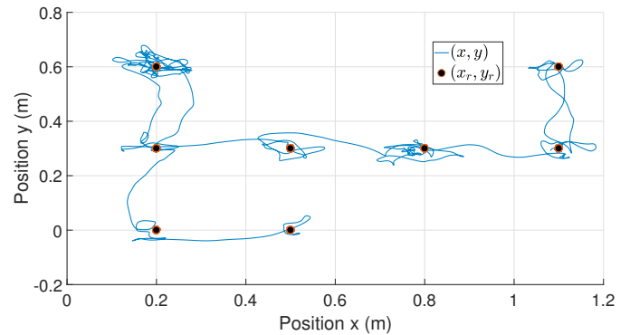
Fig. 3. Horizontal (x, y) trajectory of the uncertain system during the validation flight.
