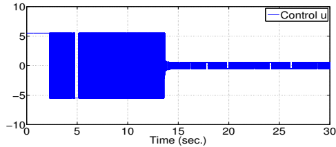
(a) control law u versus time (s).
