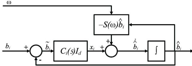
Fig. 3. Passive linearlike complementary filter.
