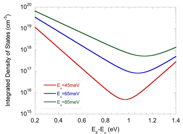
Figure 17. One-electron density of states N^{\#} integrated over energy as a function of the Fermi level position for three values of the valence band tail Urbach energy E_U .
