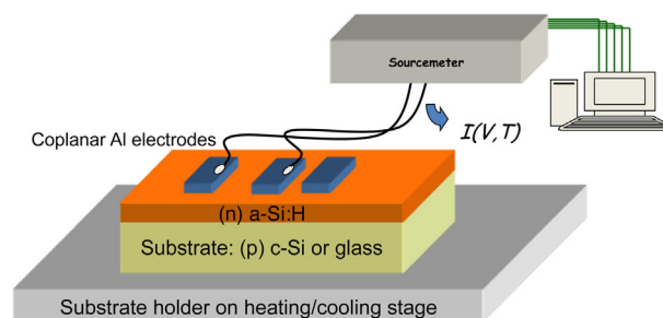
Figure 3. Measurement principle of the planar lateral conductance.
