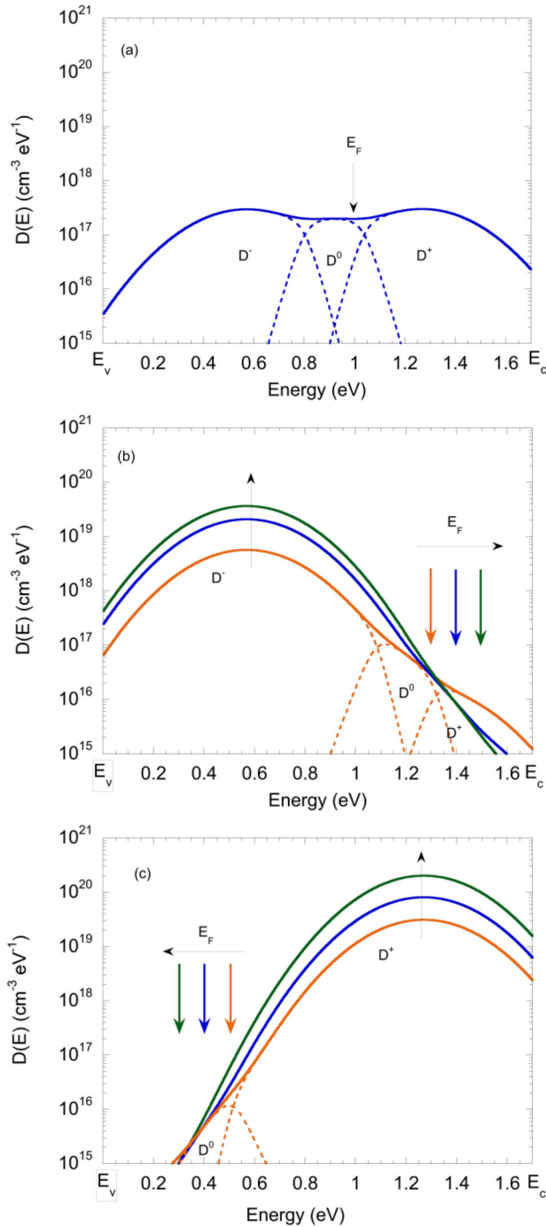
Figure 16. Calculated density of dangling bond states D(E) with defect-pool parameters [46] in undoped a-Si:H (a), n-type a-Si:H (b) and p-type a-Si:H (c) at T = 300\text{ K} ( T_{eq} = 500\text{ K} ). In n-type (p-type) a-Si:H, the Fermi level E_F is shifted by 0.3 eV (0.5 eV)-orange, 0.4 eV (0.6 eV)-blue and 0.5 eV (0.7 eV)-green from its position in undoped a-Si:H leading to a strong increase of the D^- ( D^+ ) density. For clarity of the figures, the D^- , D^0 , and D^+ components with smaller densities are only shown for one position of the Fermi level in doped a-Si:H.
