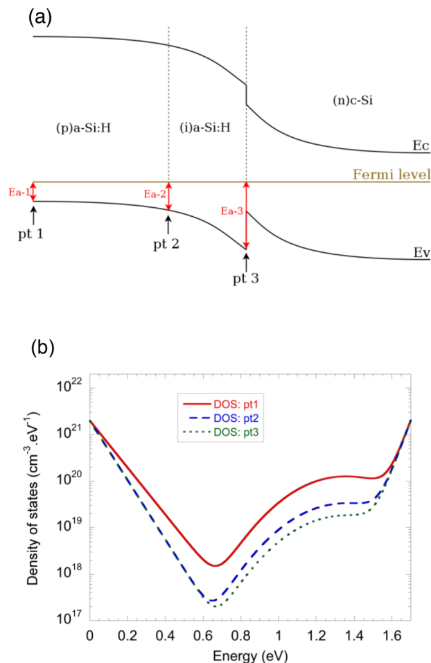
Figure 18. (a) (p) a-Si:H/(i) a-Si:H/(n) c-Si band diagram; (b) One-electron density of states in a-Si:H calculated using the defect-pool model at different points of the band diagram in (a): top of the (p) a-Si:H layer (pt 1), (p) a-Si:H/ (i) a-Si:H interface (pt 2) and (i) a-Si:H/ (n) c-Si interface (pt 3). The deep defect density has been deduced from the DB distribution calculated using the defect-pool model with parameters from Powell and Deane. [46] The Urbach energy of the valence band tail has been taken equal to 86 meV in (p) a-Si:H (pt1), and 68 meV in (i) a-Si:H (pt2 and pt3). Data from Ref. [52].
