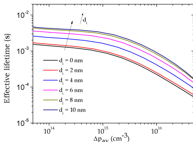
Figure 23. Simulated effective lifetime in c-Si for (p) a-Si:H/(i) a-Si:H/(n) c-Si/(i) a-Si:H/(p) a-Si:H structures equivalent to those studied experimentally taking into account the exponential variation law of the Urbach energy with thickness in the (i) a-Si:H layer.
