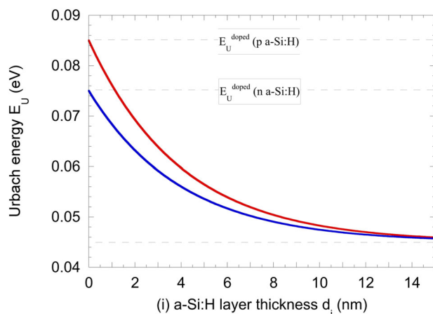
Figure 22. Exponential variation law of the Urbach energy with the (i) a-Si:H layer thickness that was integrated into our model.
