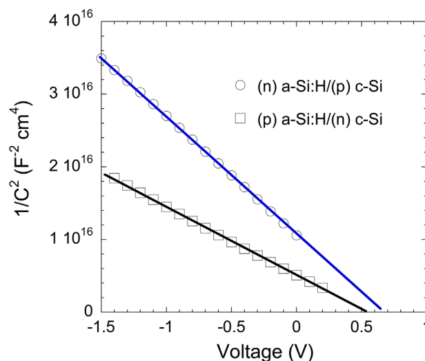
Figure 12. Voltage dependence of the inverse square capacitance (per unit area) measured on both types of heterojunctions, (n) a-Si:H/(p) c-Si and (p) a-Si:H/(n) c-Si. Full lines are linear fits to the experimental data. In each case, the slope yields the correct doping density N_{dop} that corresponds to the acceptor or donor density in c-Si, respectively.
