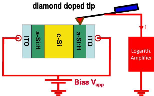
Figure 9. Sketch of the sample configuration under DC bias during the CP-AFM measurement. Both (n) a Si:H/(p) c Si/(n) a Si:H and (p) a Si:H/(n) c Si/(p) a Si:H were probed. [29] The c-Si wafer thickness was about 200 \mu\text{m} , while the a-Si:H thickness was 300 nm thick, deliberately thicker than in solar cells. Results in Figure 10 and 11 are shown for (n) a Si:H/(p) c Si/(n) a Si:H structures.
