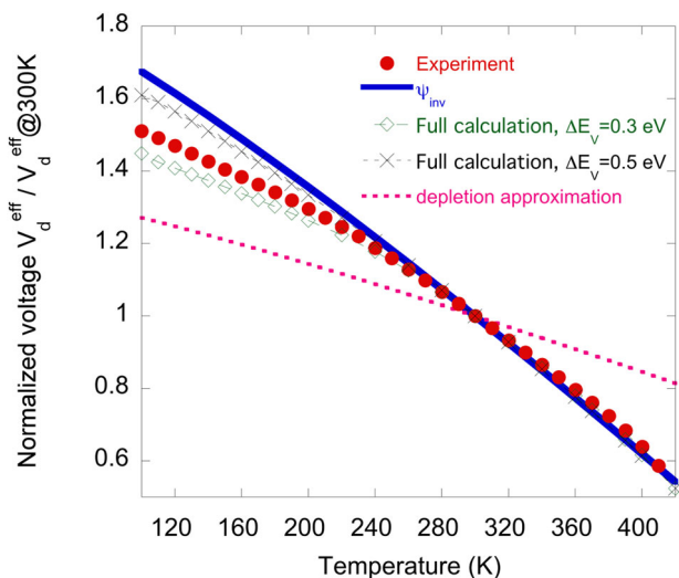
Figure 14. Effective diffusion voltage at zero DC bias, V_d^{eff} , as a function of temperature, in a P/n heterojunction. Experimental data (full dots) are compared to the band bending at the strong inversion limit, \psi_{inv} from Equation (10) (full line) and to the values obtained from the calculation using the depletion approximation (dotted lines) or from a full calculation including the contribution of carriers in the strong inversion layer for two values of valence band offset, \Delta E_V = 0.3 eV (open diamonds) and \Delta E_V = 0.5 eV (crosses). All data have been normalized to their values at 300 K. Data from Ref. [37].
