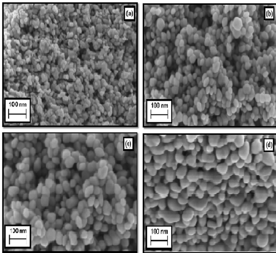
Fig. 4. SEM observation of \alpha\text{-Fe}_2\text{O}_3 prepared with different concentrations of \text{FeCl}_3 \cdot 6\text{H}_2\text{O} : (a) [\text{Fe}^{3+}] = 0.05 \text{ M} , (b) [\text{Fe}^{3+}] = 0.1 \text{ M} , (c) [\text{Fe}^{3+}] = 0.2 \text{ M} and (d) [\text{Fe}^{3+}] = 0.4 \text{ M} .
