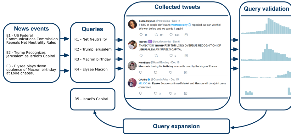
Fig. 1. Diagram of our keywords mining approach on three recent events
