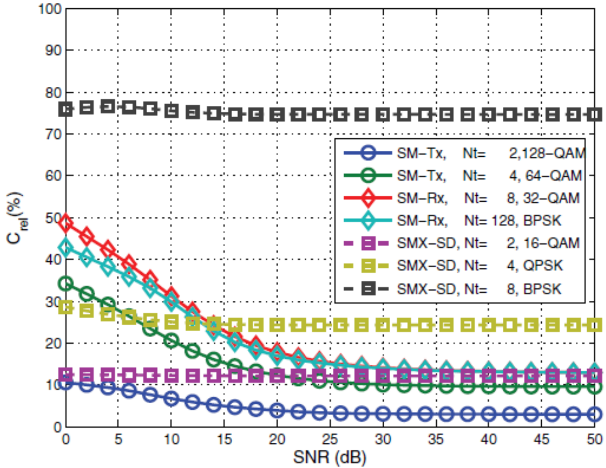
Fig. 8. Demodulation complexity. Reproduced from [40] with permission.
