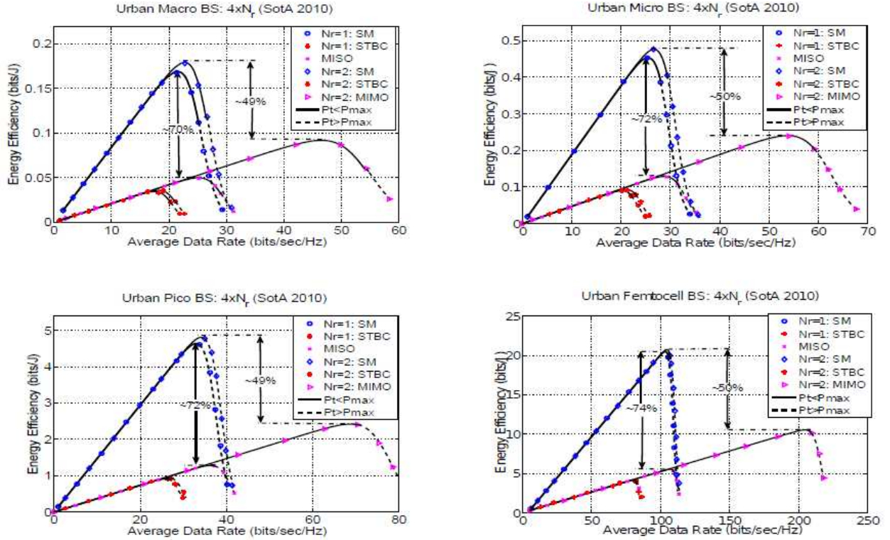
Fig. 9. Energy efficiency. Reproduced from [41] with permission.
