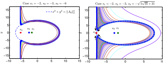
Fig. 3. Envelope curve of the characteristic equation (7). Case s_1 = -2 , s_2 = -3 , and s_3 = -R (right), and 0 > s_3 > -R (left).
