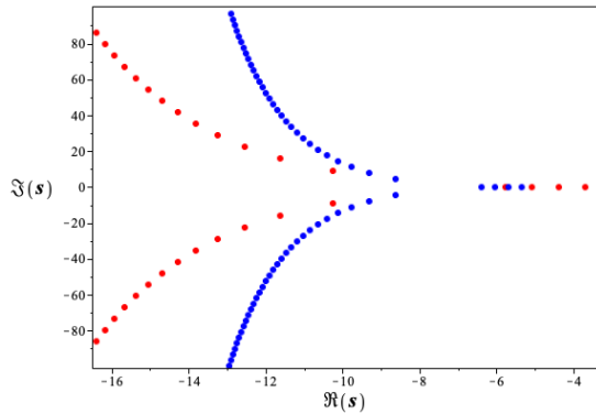
Fig. 4. The spectrum distribution of (21) satisfying (22) exhibiting the four-roots placement in two configurations. In blue, the spectrum corresponding to a = 5 , \tau = 2 . In red, the spectrum corresponding to a = 3 , \tau = 1 . In both cases, the dominance of the four assigned equidistributed real roots is underlined.
