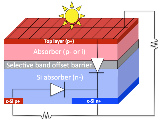
Figure 1: Three terminal band offset barrier structure showing two independent operating circuits for top and bottom cells for the case of an n-type IBC bottom cell.
