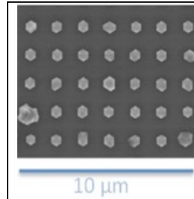
Fig. 2: Plan-view of a scanning electron microscopy (SEM) image of regularly patterned microscale GaAs crystallites on (111) Si. Underneath silica layer patterned with e-beam lithography.
