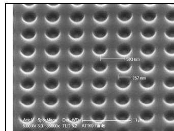
Fig. 4.1 : SEM image of an imprint in UV curable resist with PDMS flexible stamp obtained from a Si master mold, obtained at C2N (horizontal distance between two adjacent holes centers = 503 nm)
