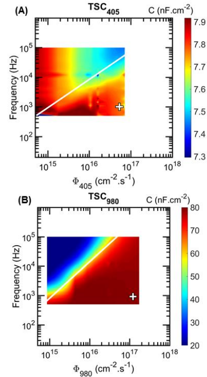
Figure 6: (A) Measured C - f - \Phi_{405} mapping for the \text{TSC}_{405} and (B) Measured C - f - \Phi_{980} mapping for the \text{TSC}_{980} . White lines represent the limit where \omega C_i \sim G_{D,i} . To emphasize the good agreement between measurements and modeling, the axe limits are defined in order to match those of Fig. 4. The white crosses show the chosen experimental conditions.
