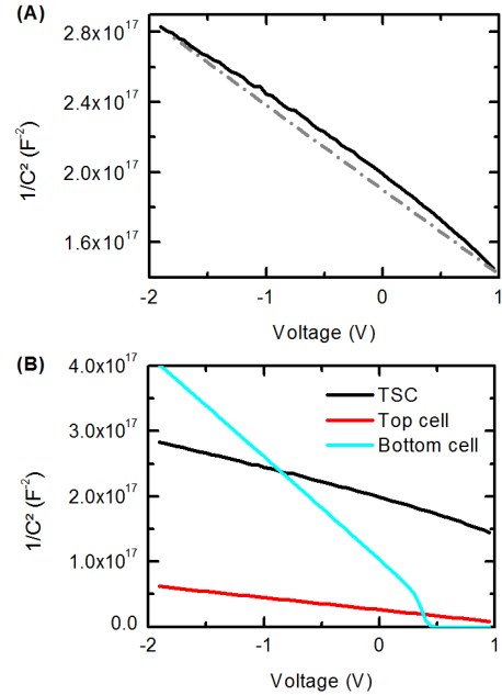
Figure 1: (A) Mott-Schottky plot obtained from numerical calculations for the TSC (black line). The dash-dotted is a straight line to show that the slope of 1/C^2 is bias dependent. (B) Mott-Schottky plots for the TSC (black line) are compared to those calculated for the subcells alone: top cell (red line) and bottom cell (blue line). Calculations were performed in the dark at T = 300 K.
