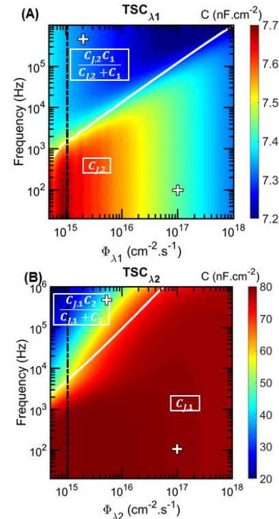
Figure 4: Mapping of the capacitance in the frequency - photon flux space ( C - f - \Phi ) for (A) the TSC _{\lambda 1} and (B) the TSC _{\lambda 2} . The black dashed lines represent the cutlines from which the curves of the TSC in Fig. 3 were obtained. The white lines highlight the evolution of the frequency value for which \omega C_i = G_{D,i} . The white crosses show the conditions taken for Fig. 5.
