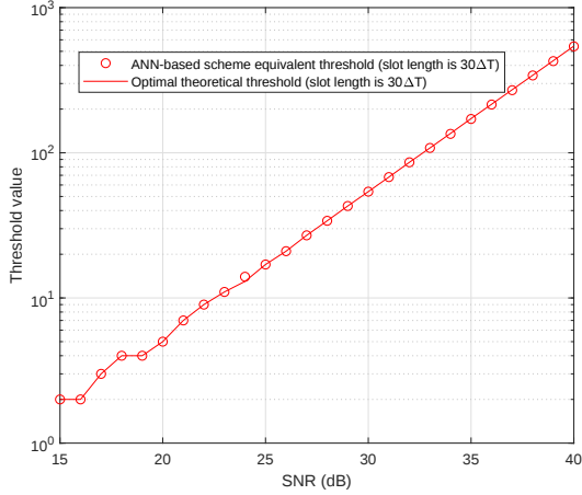
FIGURE 11: Optimal detection thresholds of model-based and data-driven schemes. The ANN-based receiver automatically emulates the optimal zero-bit memory receiver. - T = 30\Delta T .
