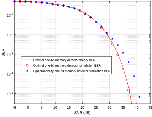
FIGURE 14: BER of optimal vs. sub-optimal one-bit memory receiver. The performance gap between optimal and sub-optimal receiver gets smaller since the ISI is modeled more accurately - T = 30\Delta T .
