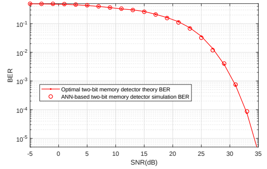
FIGURE 17: The ANN-based two-bit memory receiver achieves the same BER performance as the optimal two-bit receiver - T = 30\Delta T .
