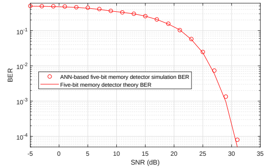
FIGURE 18: The BER performance of ANN-based and model-based L -bit memory detectors overlap with each other - T = 30\Delta T .
