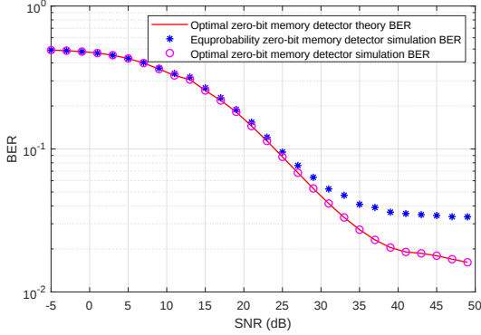
FIGURE 7: BER of optimal vs. conventional zero-bit memory receiver - T = 30\Delta T .
