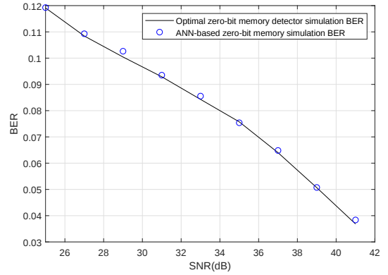
FIGURE 13: System model assuming a short distance between transmitter and receiver. The data-driven receiver achieves the same BER performance as the optimal (i.e., based on the optimal threshold) zero-bit receiver - T = 30\Delta T .
