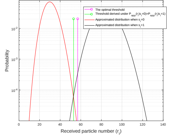
FIGURE 8: Approximated distributions of the received bits from (11) (the SNR is 25 dB).
