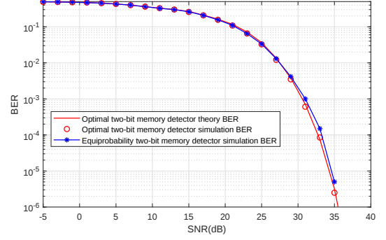
FIGURE 16: Two-bit memory detector: Comparison between the optimal and sub-optimal setups of the demodulation thresholds. The more the number of memory bits, the better the ISI is modeled. As the memory length approaches the channel length, thus, the optimal threshold converges towards the conventional threshold - T = 30\Delta T .
