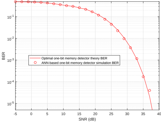
FIGURE 15: The ANN-based receiver achieves the same BER performance as the optimal one-bit receiver - T = 30\Delta T .
