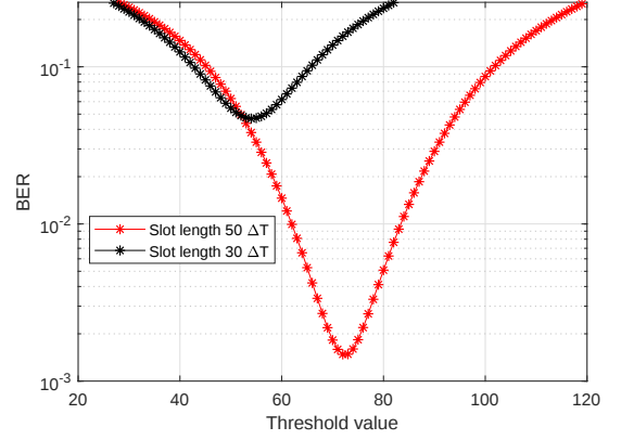
FIGURE 3: BER in (14) as a function of \tau (the SNR is 30 dB).
