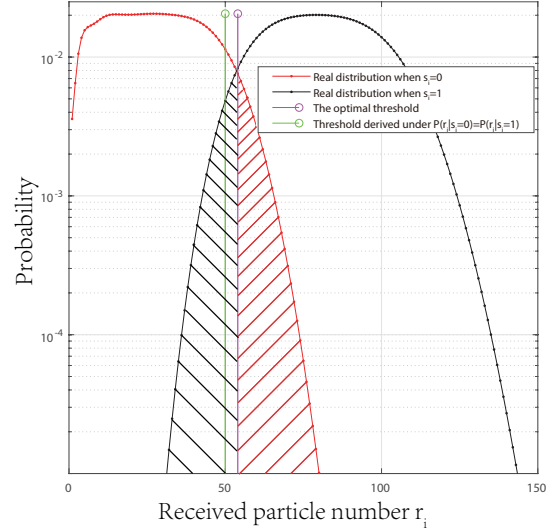
FIGURE 9: Empirical distributions of the received bits (the SNR is 25 dB).
