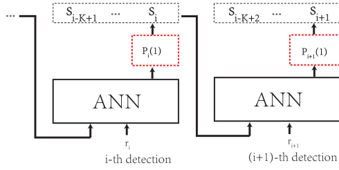
FIGURE 6: Data-driven K -bit memory receiver.
