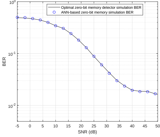
FIGURE 10: The ANN-based receiver achieves the same BER performance as the optimal zero-bit receiver - T = 30\Delta T .
