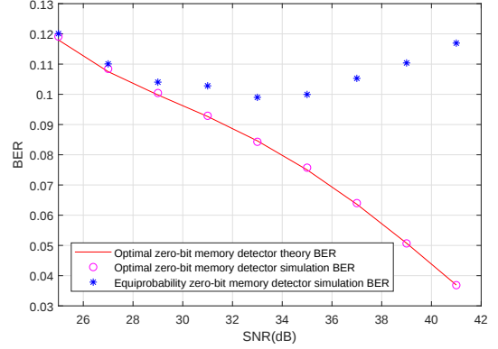
FIGURE 12: System model assuming a short distance between transmitter and receiver. BER of the optimal vs. sub-optimal (i.e., based on the sub-optimal threshold) zero-bit memory receiver - T = 30\Delta T .
