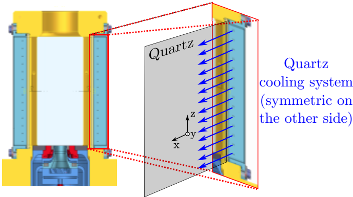
FIGURE 4. Combustion chamber quartz cooling system (from ISF communication [31])
