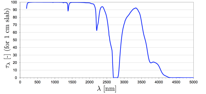
FIGURE 5. Internal transmittance of a 1 cm Corning HPFS 7980 quartz slab (from [37]).
