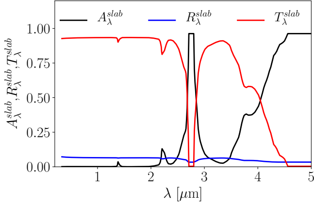
FIGURE 6. Computed quartz slab absorptance ( A_{\lambda}^{\text{slab}} ), transmittance ( T_{\lambda}^{\text{slab}} ) and reflectance ( R_{\lambda}^{\text{slab}} ) as a function of the wavelength \lambda for a 3-mm thickness. The quartz reference is Corning HPFS 7980.
