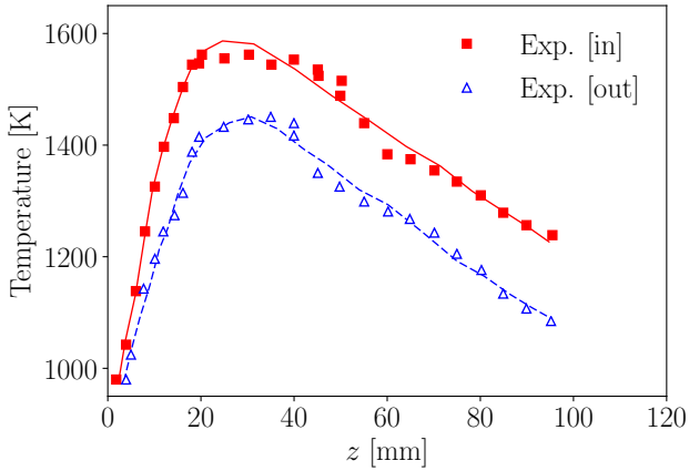
FIGURE 2. Measured temperatures of the inner and outer surface of the combustion chamber windows along the vertical axis for Case 1 [29]. Lines correspond to fits of the experimental data.
