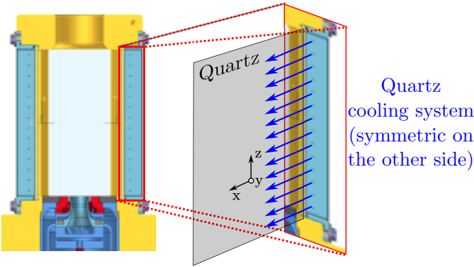
FIGURE 4. Combustion chamber quartz cooling system (from ISF communication [31])
