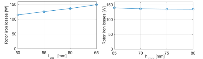
Fig. 14. Influence of machine length and rotor height on the iron losses
