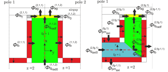
Fig. 10. left: mean flux path between two pole, right: mean flux path in a rotor flux guide
