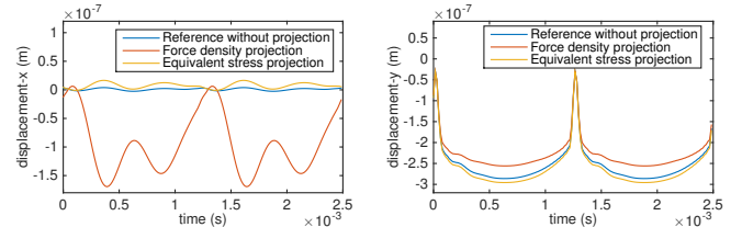
Fig. 2. Displacements as a function of time of the measure point in direction of 'x' and 'y'.
