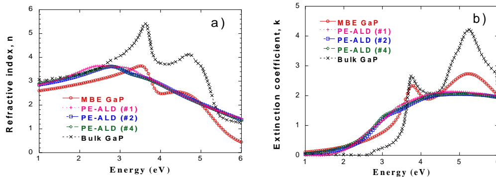
Figure 2 Experimental refractive index (a) and extinction coefficient (b) determined from spectroscopic ellipsometry for GaP layers on Si grown by MBE and PE-ALD.
