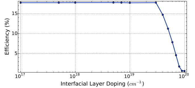
Figure 7: Efficiency as a function of the interfacial layer doping concentration, for a metal work function W_f = 6.3\text{eV} , an Indium composition of x = 0.56 , a doping of N_d = 6.5 \times 10^{16}\text{cm}^{-3} and an InGaN layer thickness of T_{\text{InGaN}} = 0.86\mu\text{m} .
