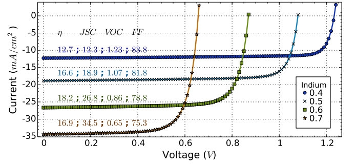
Figure 5: Current - Voltage characteristic for for different Indium compositions x , for a metal work function W_f = 6.3 \text{eV} , a doping of N_d = 6.5 \times 10^{16} \text{cm}^{-3} and an InGaN layer thickness of T_{\text{InGaN}} = 0.86 \mu\text{m} . \eta , JSC, VOC and FF are respectively abbreviations for Efficiency (%), Short-Circuit current density ( \text{mA}/\text{cm}^2 ), Open-Circuit voltage (V) and Fill Factor.
