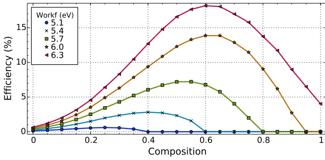
Figure 3: Efficiency as a function of the Indium compositions x for different metal work function W_f , for a doping of N_d = 6.5 \times 10^{16} \text{cm}^{-3} and an InGaN layer thickness of T_{\text{InGaN}} = 0.86 \mu\text{m} .
