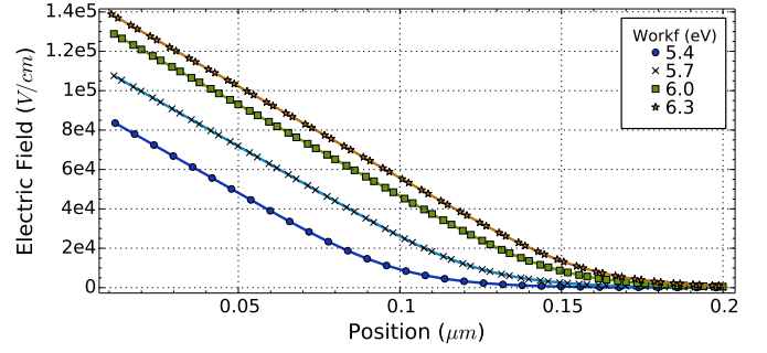
Figure 4: Electric field as a function of the distance from the device surface for different metal work function W_f , for a doping of N_d = 6.5 \times 10^{16} \text{cm}^{-3} , an Indium composition of x = 0.56 and an InGaN layer thickness of T_{\text{InGaN}} = 0.86 \mu\text{m} .
