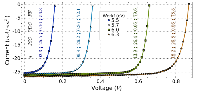
Figure 6: Current - Voltage characteristic for different work functions, for an Indium composition of x = 0.56 , a doping of N_d = 6.5 \times 10^{16} \text{cm}^{-3} and an InGaN layer thickness of T_{\text{InGaN}} = 0.86 \mu\text{m} . \eta , JSC, VOC and FF are respectively abbreviations for Efficiency (%), Short-Circuit current density ( \text{mA}/\text{cm}^2 ), Open-Circuit voltage (V) and Fill Factor.
