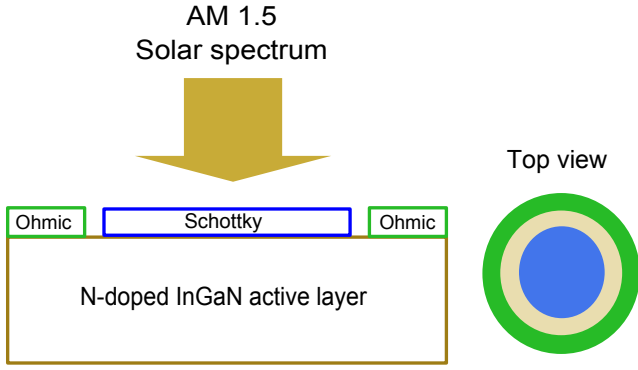
Figure 1: InGaN solar cell device structure.
