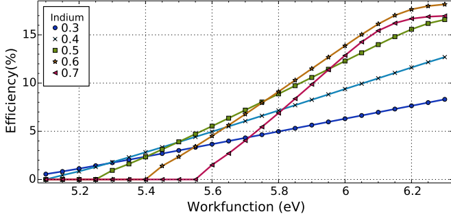
Figure 2: Efficiency as a function of the metal work function W_f for different Indium compositions x , for a doping of N_d = 6.5 \times 10^{16} \text{cm}^{-3} and an InGaN layer thickness of T_{\text{InGaN}} = 0.86 \mu\text{m} .
