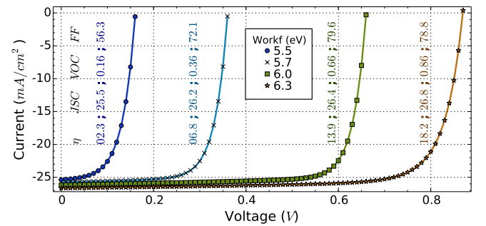
Figure 6: Current - Voltage characteristic for different work functions, for an Indium composition of x = 0.56 , a doping of N_d = 6.5 \times 10^{16} \text{cm}^{-3} and an InGaN layer thickness of T_{\text{InGaN}} = 0.86 \mu\text{m} . \eta , J_{SC} , V_{OC} and FF are respectively abbreviations for Efficiency (%), Short-Circuit current density ( \text{mA}/\text{cm}^2 ), Open-Circuit voltage (V) and Fill Factor.
