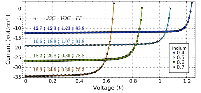
Figure 5: Current - Voltage characteristic for for different Indium compositions x , for a metal work function W_f = 6.3 \text{eV} , a doping of N_d = 6.5 \times 10^{16} \text{cm}^{-3} and an InGaN layer thickness of T_{\text{InGaN}} = 0.86 \mu\text{m} . \eta , J_{SC} , V_{OC} and FF are respectively abbreviations for Efficiency (%), Short-Circuit current density ( \text{mA}/\text{cm}^2 ), Open-Circuit voltage (V) and Fill Factor.
