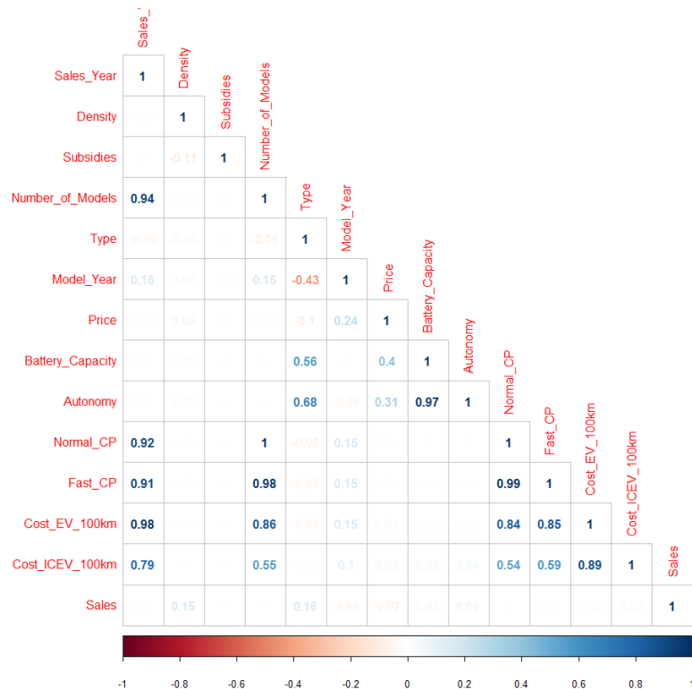
Fig. 7. Mutlicolnearity between the model's variables
