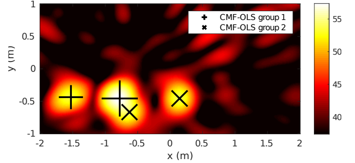
FIG. 10. Experimental results with two pairs of correlated sources at F = 2.2 kHz. The sources identified by CMF-OLS are superimposed over the output of the standard beamformer.
