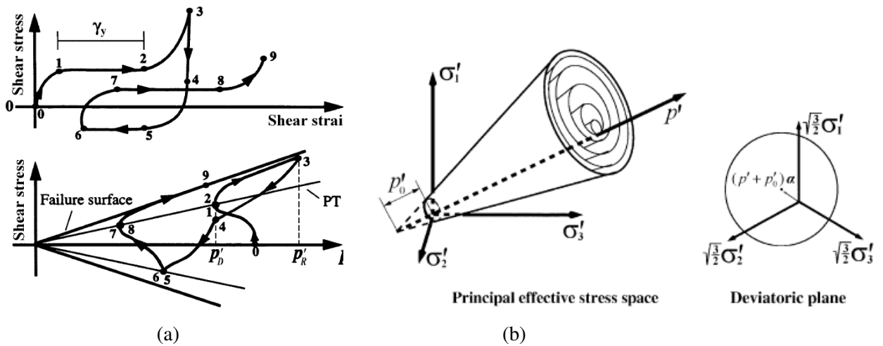
Figure 3: a) Schematic of constitutive model response showing shear stress, effective confinement, and shear strain relationship, b) Conical yield surface in principal stress space and deviatoric plane (after Prevost [22], Parra [21], Yang and Elgamal [28]).
