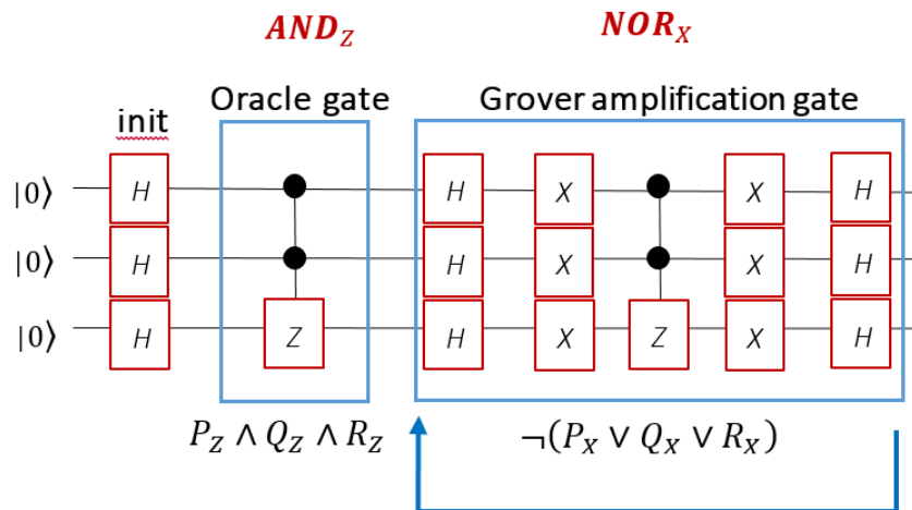
Figure 1. Quantum circuit for the phase oracle followed by the Grover amplification gate interpreted as a first-order existential proposition using Eigenlogic AND and OR operators.
