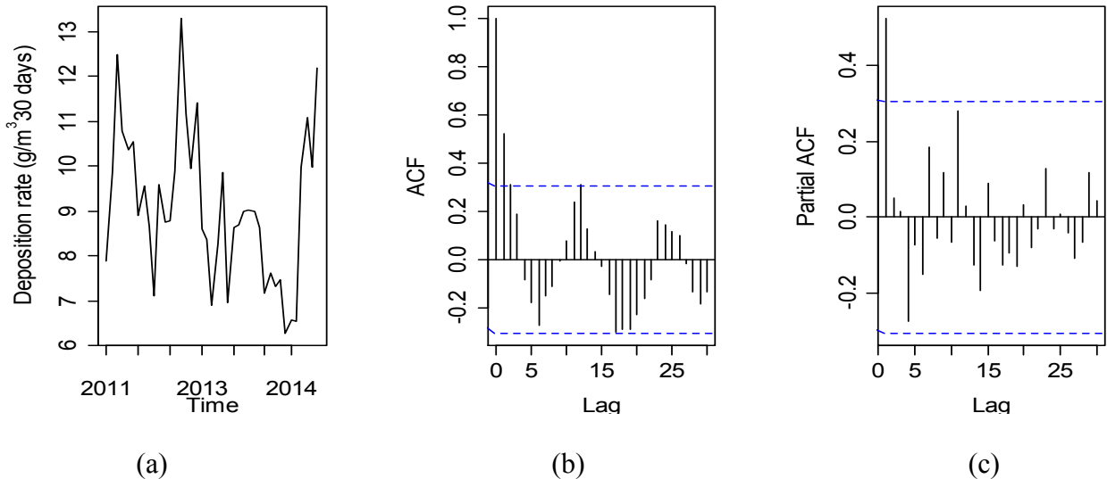
Figure 2 – Time series (a), autocorrelation function (b) and partial autocorrelation function (c) for SPM from 2011 to 2014.
