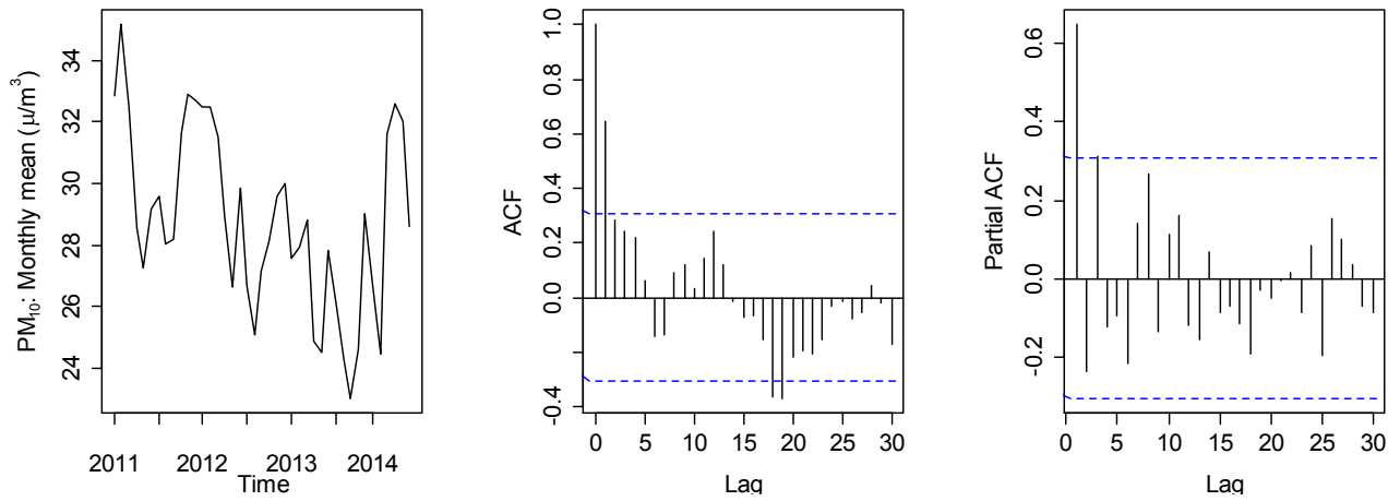
(a) (b) (c) Figure 3- Time series (a), autocorrelation function (b) and partial autocorrelation function (c) for monthly mean concentration of PM_{10} from 2011 to 2014.
