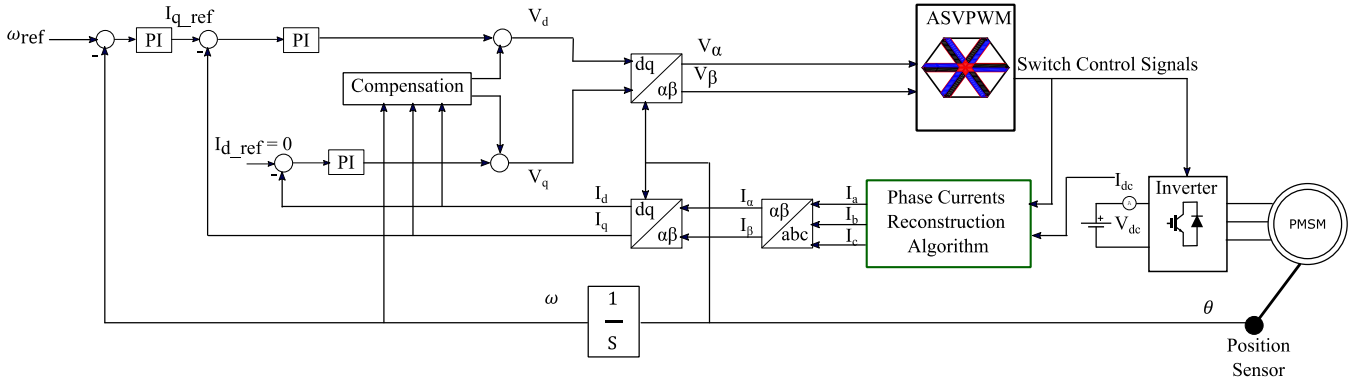
Fig. 2. Overview of the control system with DC Bus current
