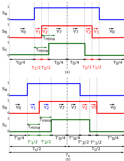
Fig. 12. Switching control signal for a reference vector with a low modulation index applying in sector 1: (a) with Standard SVPWM, (b) With Adjusted SVPWM
