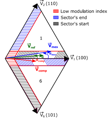
Fig. 7. Reference vector applying at the beginning of sector 1
