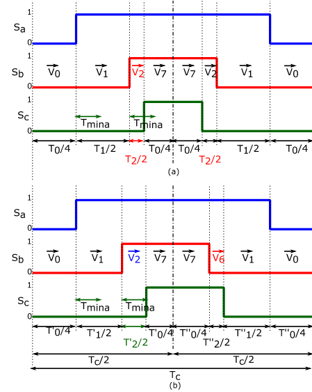
Fig. 8. Switching control signal applying at the start of sector 1: (a) with Standard SVPWM, (b) With Adjusted SVPWM
