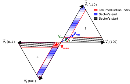
Fig. 11. Reference vector with a low modulation index applying in sector 1
