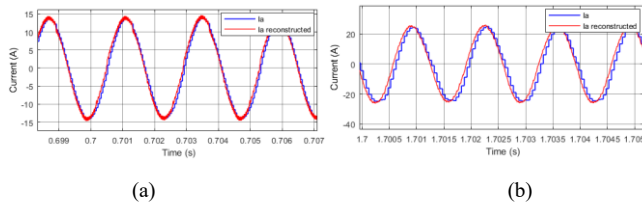
Fig. 16. Comparison between reconstructed current and the current obtained via simulation of the phase a: (a) at 5000 rpm, (b) at 9000 rpm
