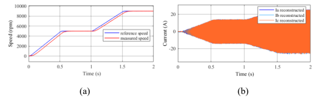
Fig. 14. (a) PMSM speed with f_{sw}=20 kHz, (b) reconstructed phase currents
