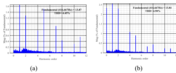
Figure 17 : (a) spectrum of phase currents obtained via simulation at 5000 rpm, (b) spectrum of reconstructed phase currents at 5000 rpm
