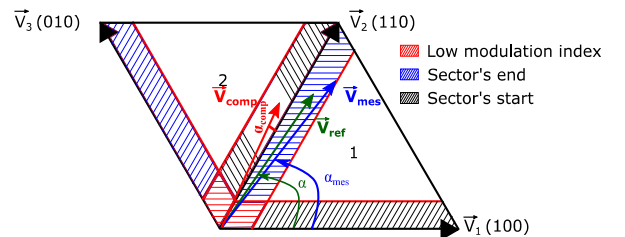
Fig. 9. Reference vector applying at the end of sector 1
