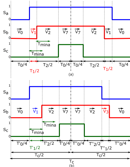
Fig.10. Switching control signal applying at the end of sector 1: (a) with Standard SVPWM, (b) With Adjusted SVPWM
