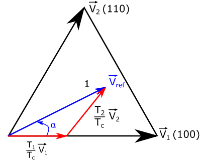
Fig. 4. Reference vector applying in sector 1
