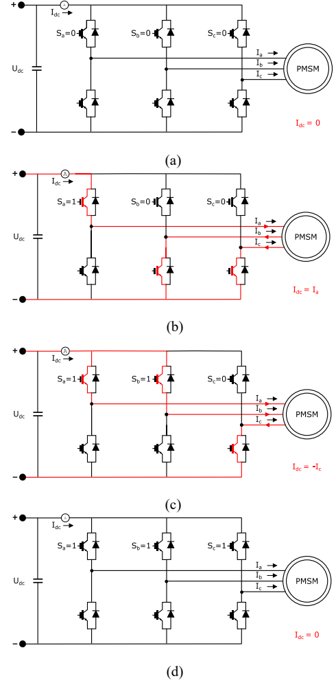
Fig. 6. Current under different voltage vectors applying in sector 1: (a) V_0 applied, (b) V_1 applied, (c) V_2 applied, (d) V_7 applied.
