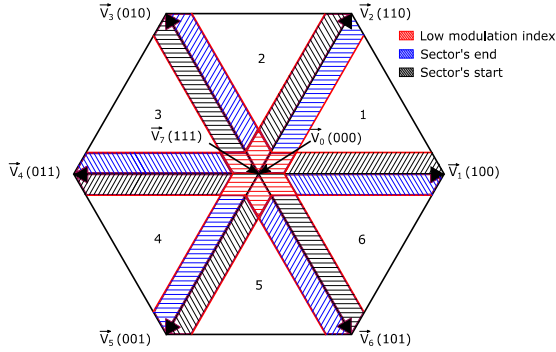
Fig. 3. Vectors and sectors of SVPWM
