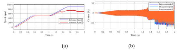
Fig. 13 : (a) PMSM speed with f_{sw}=10 kHz, (b) reconstructed phase current
