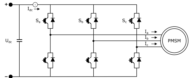
Fig. 1. Three phase inverter
