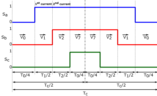
Fig. 5. Distribution of the voltage vectors in the sector n^\circ 1
