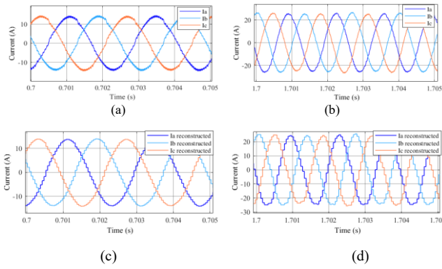
Fig. 15. Phase currents: (a) current obtained via simulation at 5000 rpm, (b) currents obtained via simulation at 9000 rpm (c) Reconstructed current at 5000 rpm, (d) reconstructed current at 9000 rpm
