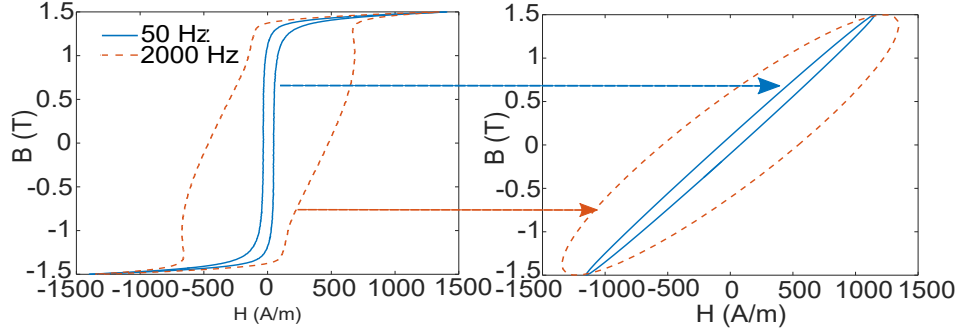
Figure 3: Conversion of non-linear hysteresis characteristics to linear-elliptical hysteresis loops at 1.5 T
