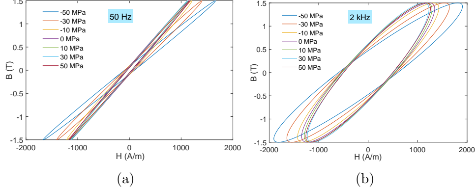
Figure 7: Linear-elliptical hysteresis loops for different stress levels at (a) 50 Hz (b) 2 kHz at 1.5 T
