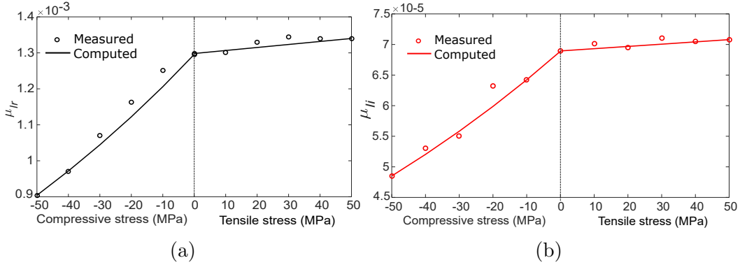
Figure 5: Variation of (a) real part of \mu_l (b) imaginary part of \mu_l with stress at 1.5 T
