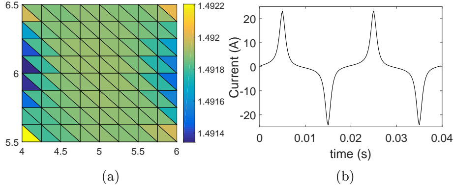
Figure 9: Simulation results (a) surface plot of flux density of the sample region shown in Fig. 8b (b) the computed current waveform
