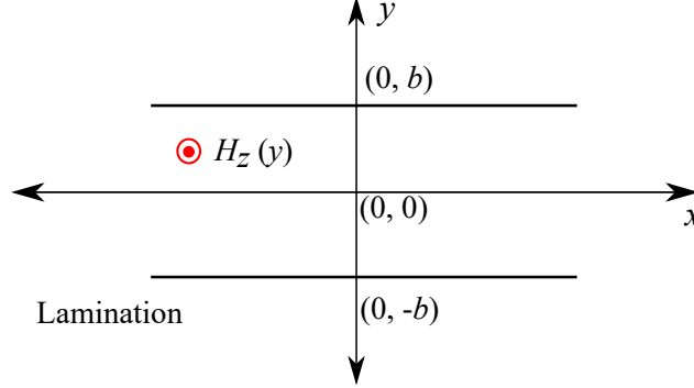
Figure 2: Semi-infinite single sheet in z -direction with x dimensions much greater than the y dimensions
