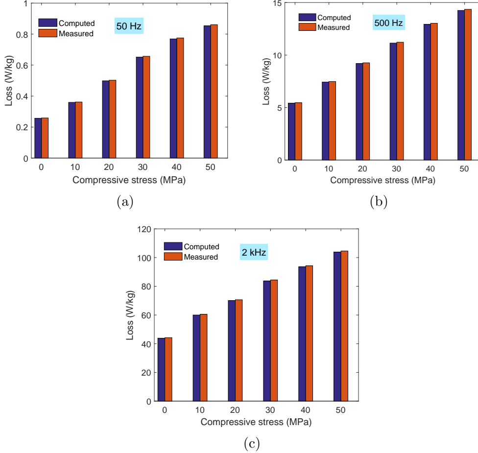
Figure 12: Comparison of measured and calculated loss using time-harmonic FEM for induction level of 0.5 T (a) 50 Hz (b) 500 Hz (c) 2 kHz
