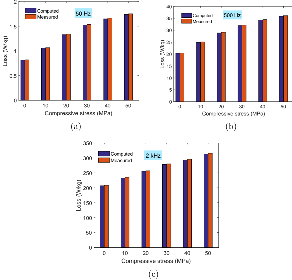
Figure 13: Comparison of measured and calculated loss using time-harmonic FEM for induction level of 1.0 T (a) 50 Hz (b) 500 Hz (c) 2 kHz
