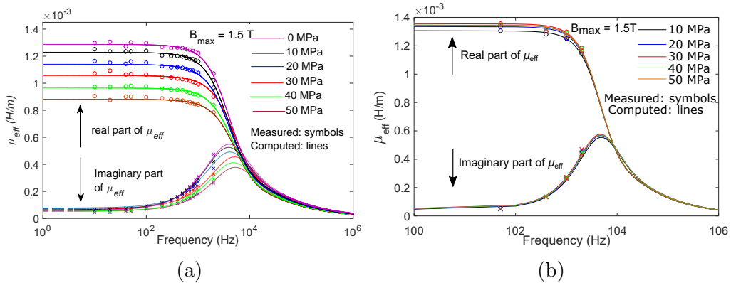
Figure 6: Variation of complex permeability at 1.5 T as a function of frequency at different stress levels (a) compressive stress (b) tensile stress
