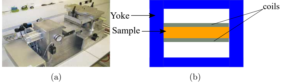
Figure 8: (a) SST with a unit to apply mechanical stresses [7] (Source: RENAULT-SAS, Guyancourt, France) (b) Geometric overview of SST
