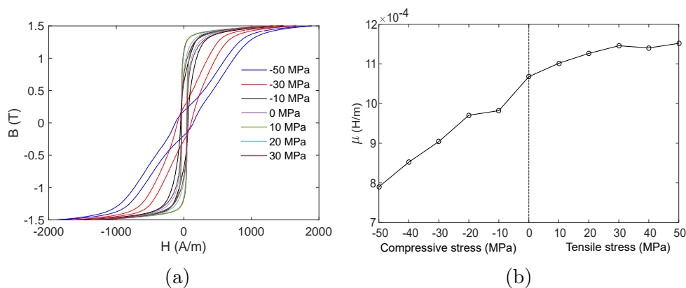
Figure 1: Variation of (a) Hysteresis loops at 1.5 T, 50 Hz for different stresses levels [7] (b) Permeability at different stress levels at 1.5 T, 50 Hz
