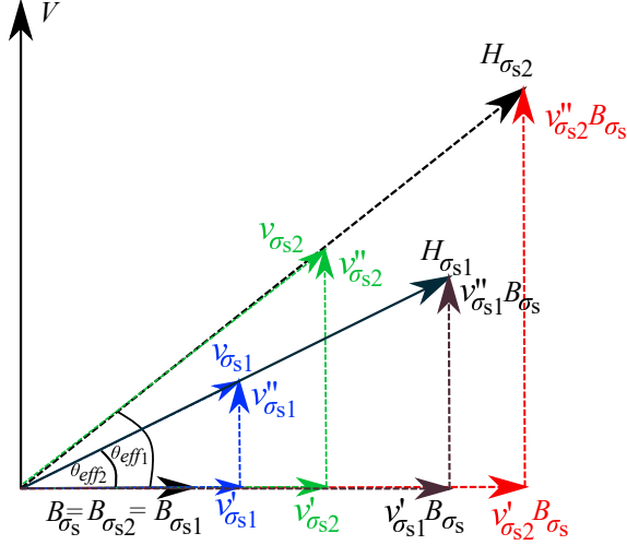
Figure 4: Phasor representation of B , H , and complex reluctivity at two different stress levels (Compressive stress: \sigma_{s1} < \sigma_{s2} and Tensile stress: \sigma_{s1} > \sigma_{s2} )
