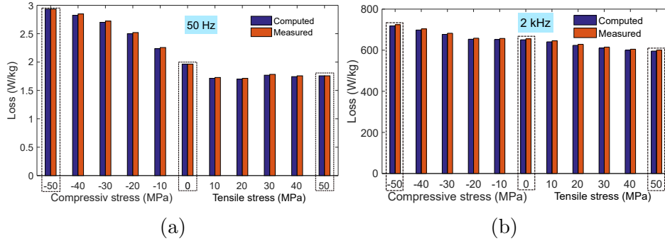
Figure 11: Comparison of measured and calculated loss using time-harmonic FEM for induction level of 1.5 T (a) 50 Hz (b) 2 kHz
