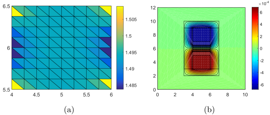
Figure 10: Simulation results (a) surface plot of flux density of the sample region shown in Fig. 8b (b) flux lines
