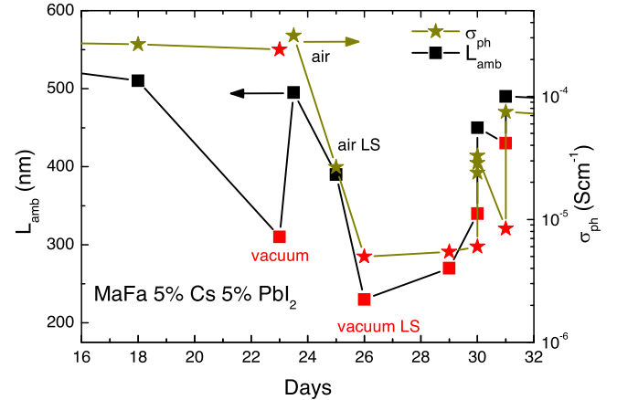
Fig. 8. Evolution of the diffusion length (squares) and of the photoconductivity (stars) of a PVK thin film with its environment (air or vacuum (red symbols)) and with light-soaking. Lines are guides to the eye.
