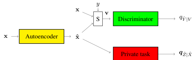
Fig. 1: Architecture (S is the selector block).
