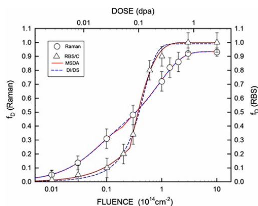
Fig. 16 Damage fraction ( f_D ) deduced from Raman and RBS/C spectra of 6H-SiC as a function of the 4.0-MeV Au ion fluence with the fits using the Multi Step Damage Accumulation (MSDA, solid line) and the DI/DS (Double Impact-Defect Stimulated, dashed line) models. Reproduced with permission from the publisher (Taylor & Francis Ltd, http://www.tandfonline.com ). Miro S., Costantini, J.-M., Huguet-Garcia, J., Thomé, L., 2014. Recrystallization of hexagonal silicon carbide after gold ion irradiation and thermal annealing. Philos. Mag. 94 (34), 3898–3913.
