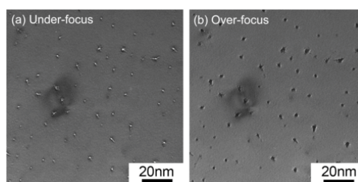
Fig. 6 Plan-view microstructures from BFTEM images of an identical region in \text{CeO}_2 irradiated at ambient temperature with 210 MeV Xe ions to a fluence 1 \times 10^{12} \text{ cm}^{-2} , taken with a kinematical diffraction condition with under-focus (a) and over-focus (b) conditions to observe the core damage regions of ion tracks with Fresnel-contrast. Reproduced with permission from Yasuda, K., Etoh, M., Sawada, K., et al. , 2013. Nucl. Instrum. Method B 314, 185–190.
