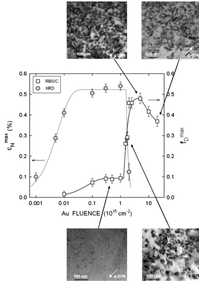
Fig. 4 Maximum damage fraction ( f_D^{\max} ) and elastic strain ( \epsilon_N^{\max} ) in YSZ single crystals (9.5 mol% Y_2O_3 ) obtained from RBS/C and XRD as a function of 4 MeV Au ions. TEM images showing dot contrast, dislocation loops and dislocation networks are inserted to the corresponding data points. Lines are derived from the multi-step damage accumulation model. Reproduced with permission from Moll, S., Thomé, L., Sattonnay, G., et al. , 2009. J. Appl. Phys. 106 (7), 073509. Shiiyama, K., Yamamoto, T., Takahashi, T., et al. , 2010. Nucl. Instrum. Methods B 268 (19), 2980–2983.
