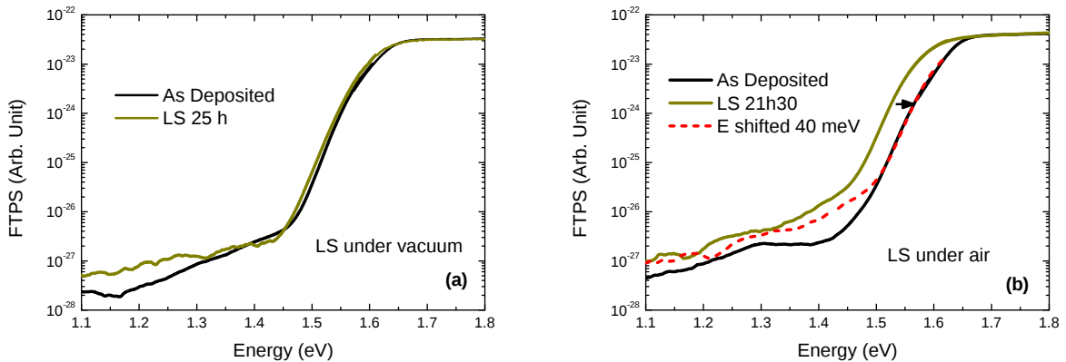
Figure 6. Evolution of the FTPS spectra with light soaking (a) performed under vacuum (b) performed under air. The FTPS spectrum obtained after light-soaking under air has been sifted 40 meV upward (dashed red line) to be compared with the as-deposited spectrum.
