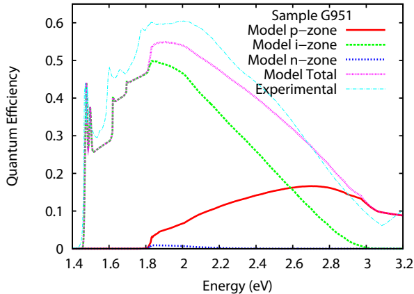
Figure 3. Experimental and modeled IQE for G951 QWSC. The contributions from p, i, and n layers are separated.
