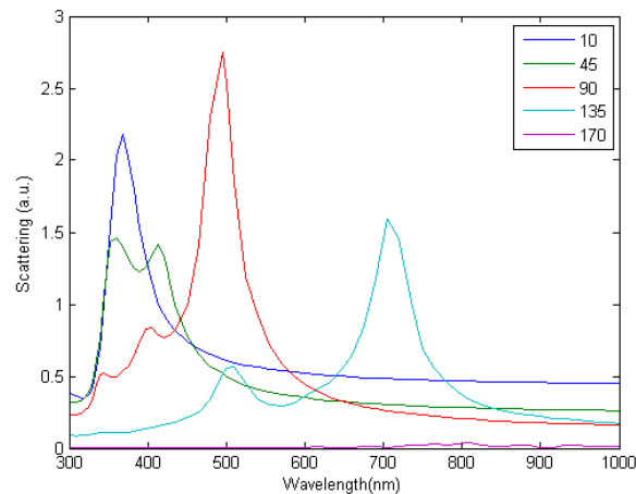
Figure 6 Numerical solution for the scattering spectra of a truncated Ag NP on a 65nm-185 \mu m SiO 2 /Si substrate, with normal incident light.
