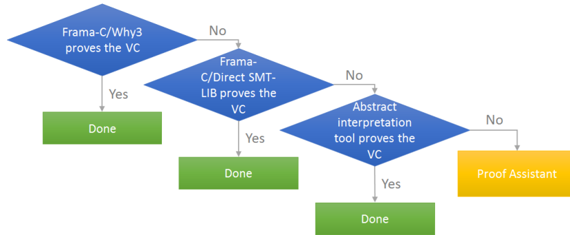
Figure 7: Methodology for proving Discrete-Valued Functions
