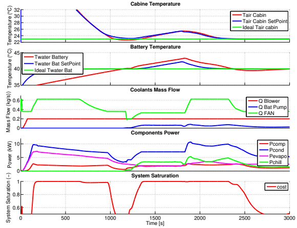
Figure 10: Functional model simulation with global supervisor control.
