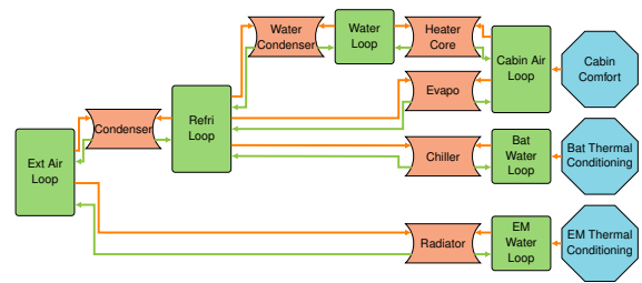
Figure 6: Electric vehicle thermal management diagram.
