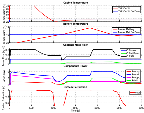
Figure 9: Functional model simulation with constant temperature setpoints.
