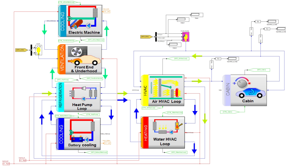
Figure 8: Electric vehicle thermal management multi-physical model.
