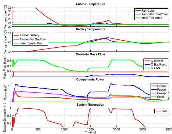
Figure 11: Multi-physical model simulation controlled by adapted functional model, itself monitored by a global supervisor.
