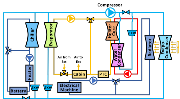
Figure 5: Diagram of electric vehicle cooling and heating circuits.
