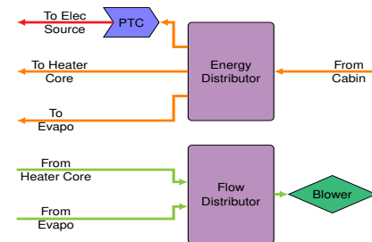
Figure 7: Cabin air loop.
