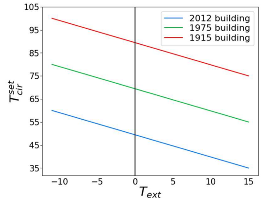
Figure 6. Heating curves used to set the heating water temperature (out of night-time set-back).
