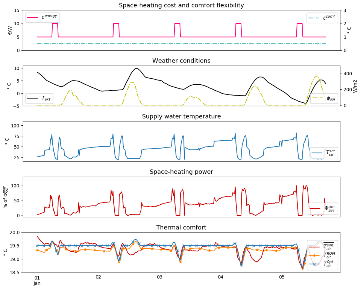
Figure 11. Space-heating MPC considering energy price variations and flexible comfort
