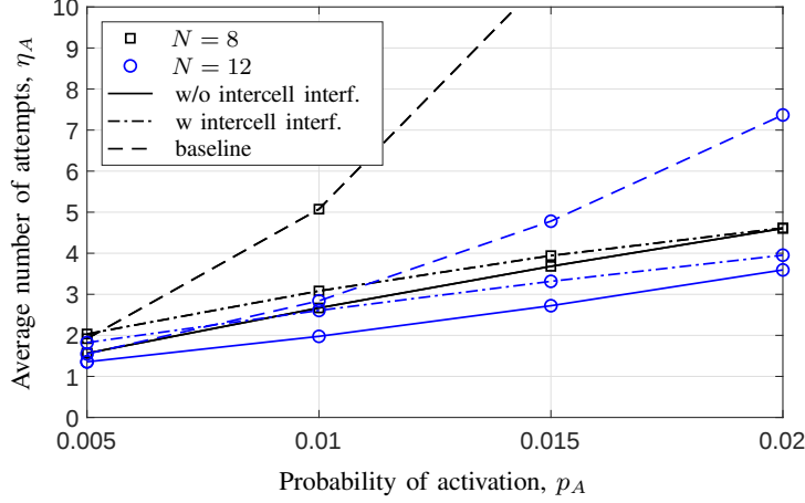
Fig. 7: Average number of attempts required by a given UE to be successfully detected with Q = 2 , N = 8 or 12, and M = 100 . Both cases with and without intercell interference are considered with uncorrelated Rayleigh fading.
