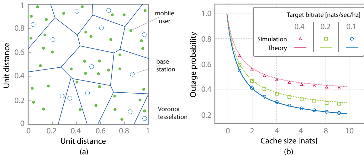
Figure 4: An example of base station deployment with caching capabilities [23]: (a) illustrates a snapshot of 2D topology in which users and cache-enabled base stations are distributed according to Poisson Point Processes (PPPs), (b) shows theoretical performance gains of such a deployment, where the validation of results is done via simulations.
