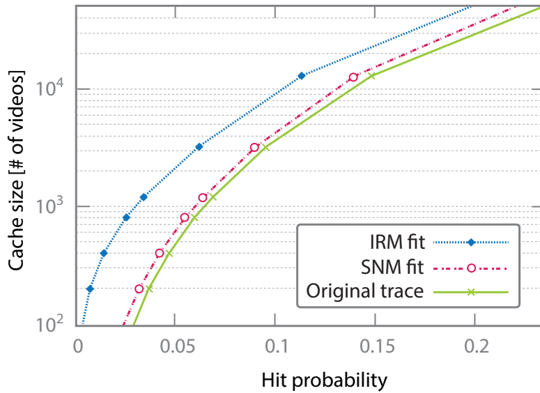
Figure 2: (from [6]) Hit probability comparison between best fit of IRM, SNM and the YouTube traces.
