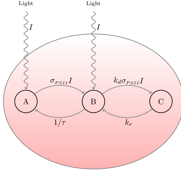
Figure 5: Schematic representation of Han's model. Red ellipse: cell. Circle: photosystem. A: open state, B: processing state, C: photodamaged state [39]
