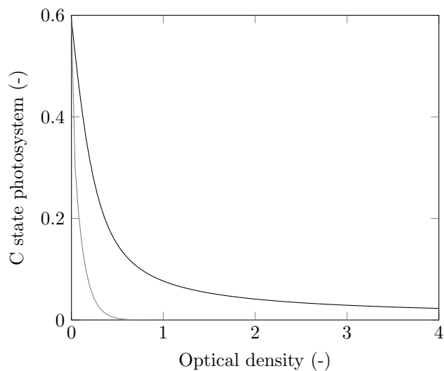
Figure 11: Fraction of the photodamaged photosystems at the population level. Light intensity: 2 000 \mu\text{molPhoton}/\text{m}^2/\text{s} . Black line: stirrer set at 100 rpm. Gray line: stirrer set at 50 rpm
