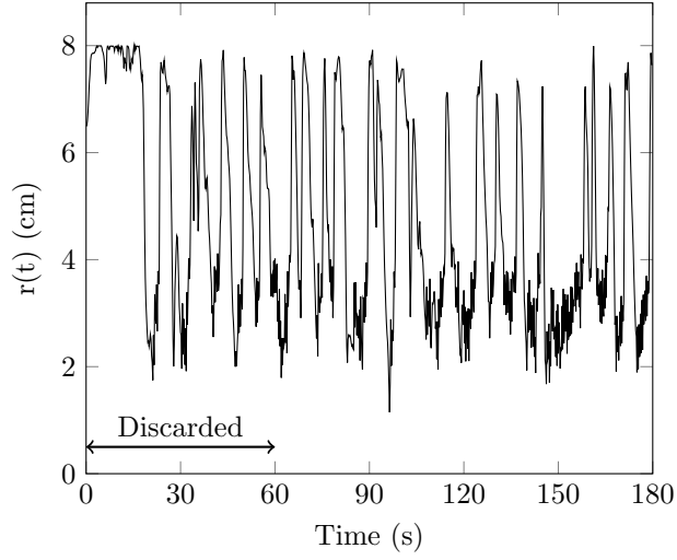
Figure 4: Radial position of a randomly drawn tracer over the first 3 minutes of computation with a stirrer set at 100 rpm
