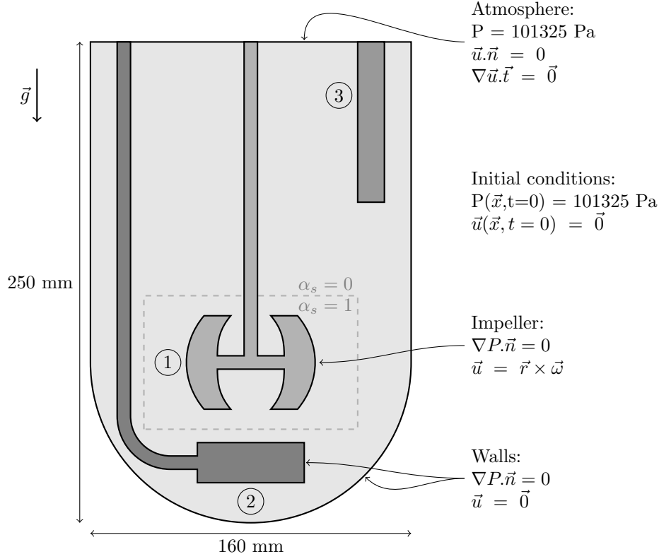
Figure 2: Case geometry with initial and boundary conditions. Aeration: 0.1 vvm, stirring: 100 rpm. 1: stirred, 2: sparger, 3: pH probe. Dashed delimited: area where the momentum source term is applied to emulate stirrer motion
