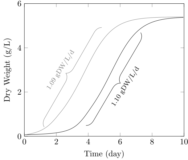
Figure 10: Predicted microalgal density inside of the reactor. Black line: two steps lighting strategy - 500 \mu\text{molPhoton}/\text{m}^2/\text{s} until an optical density of 1.0 is reached, 2 000 afterwards -. Gray line: optimal lighting strategy. Initial optical density: 0.05 / Initial dry weight: 0.1 g/L
