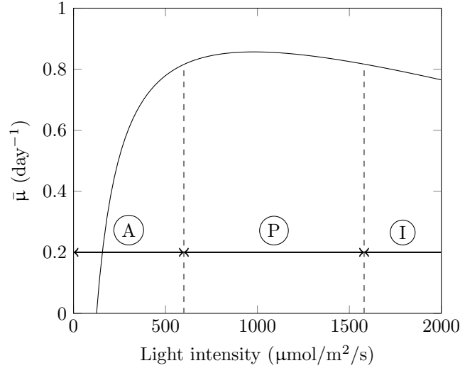
Figure 8: Population level growth at a given optical density and varying incident light intensity. Optical density: 1.0. A: affinity phase, P: plateau phase, I: inhibition phase. Number of tracer: 4 000. Integration time: 5.0 minutes
