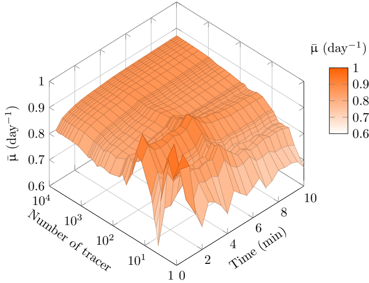
Figure 6: Population level growth rate versus integration time and number of tracers. Optical density: 1.0. Light intensity: 1 000 \mu\text{molPhoton}/\text{m}^2/\text{s}
