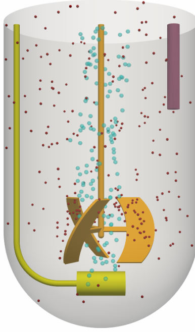
Figure 3: Visualization of the photobioreactor. Aeration: 0.1 vvm, stirring: 100 rpm. Lagrangian tracers: 10 000, only 100 represented (randomly drawn). Time: 1 minute. Color legend: blue - bubbles, red - tracers, orange - stirrer, yellow - sparger, purple - pH probe
