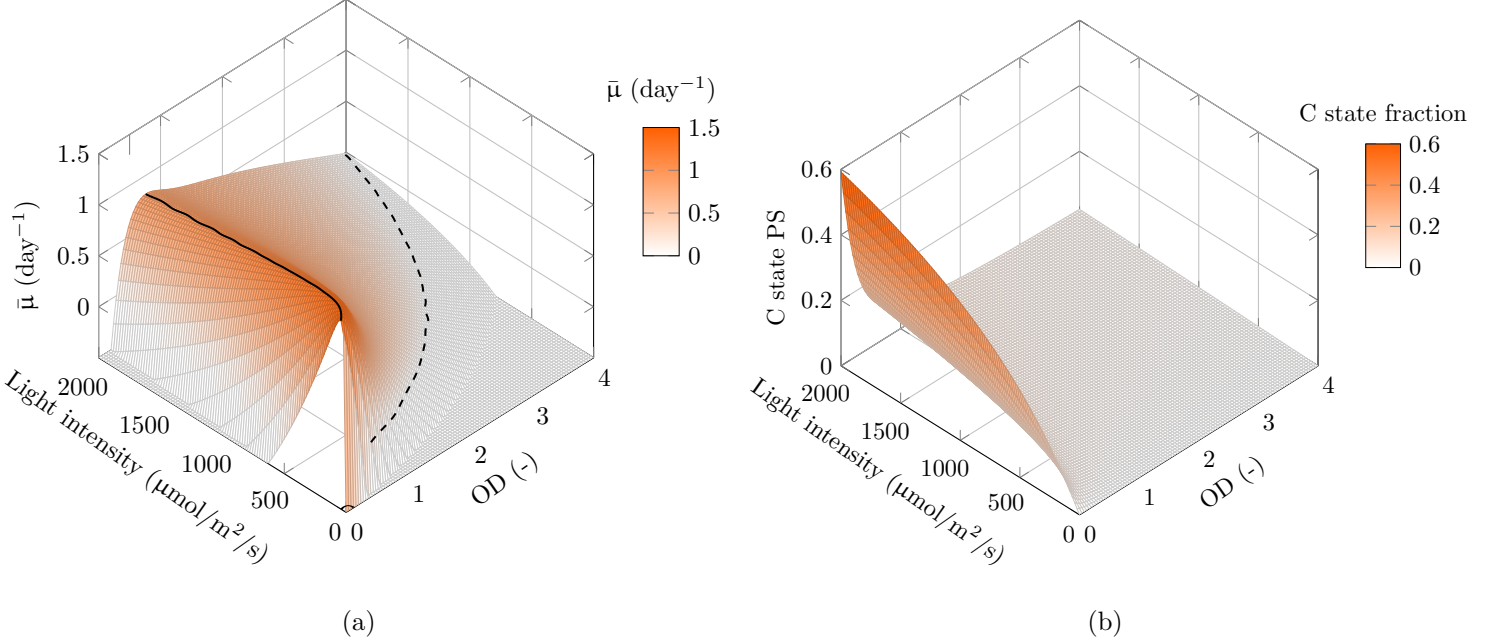
Figure 7: Population level growth rate (a) and experienced photodamages (b) versus optical density and incident light intensity. Continuous line: growth rate crest path. Dashed line: null growth rate. Number of tracer: 4 000. Integration time: 5.0 minutes
