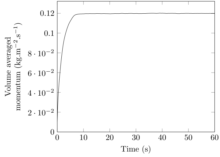
Figure 12: Volume averaged momentum. Aeration: 0.1 vvm, stirring: 100 rpm
