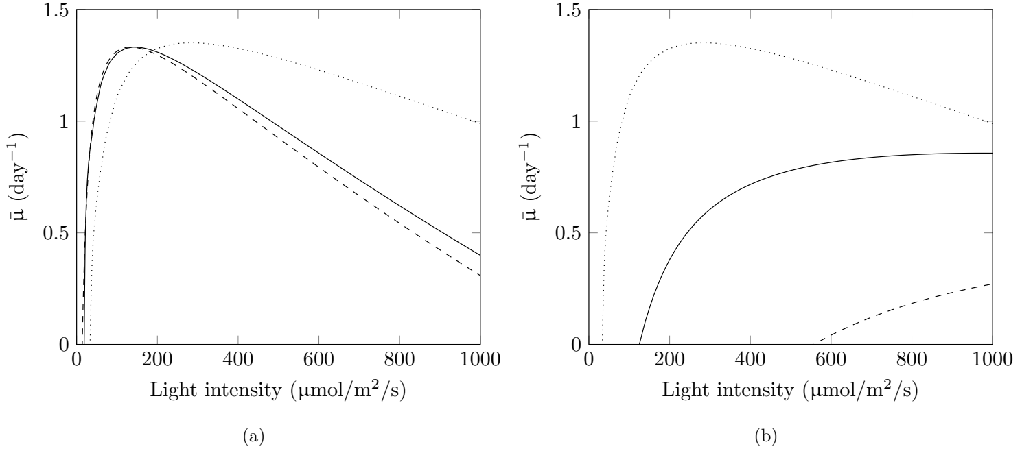
Figure 9: Population level growth rate at versus incident light intensity, at an OD of 0.2 (a) and 1.0 (b). Solid line: taking cells motion into account, dashed line: Han's model applied locally without taking microalgae motion into account, dotted line: Han's model applied only using incident light intensity and without taking microalgae motion into account
