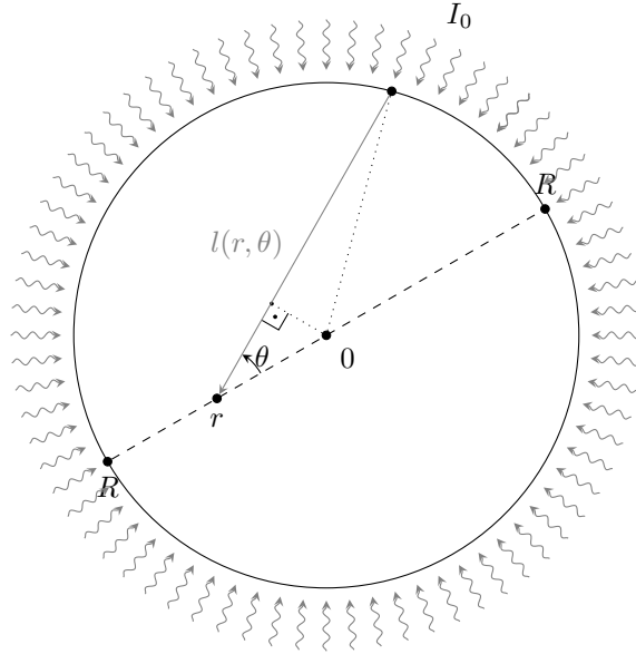
Figure 13: Light attenuation in a cylindrical geometry
