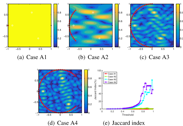
FIGURE 2. (Example 2) Maps of \mathfrak{F}_{\text{DSM}}(\mathbf{z}) and Jaccard index with f_0 = 1 GHz, where the red points represent \theta_n .
