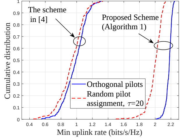
Figure 5. The cumulative distribution of the min uplink rate with proposed user assignment scheme in Section IX, with orthogonal and random pilots for M = 120 , K = 30 , K_m = 20, \forall m , and D = 1 \text{ km}^2 .
