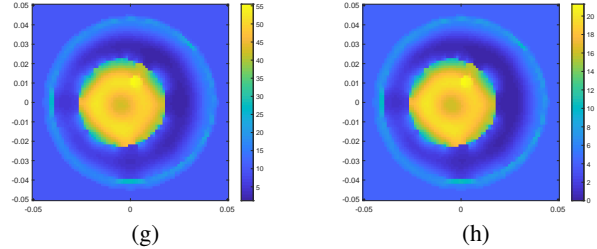
Fig. 4: Retrieved real (left) and imaginary (right) parts of Model 1. (a),(b) DBIM-UGS; (c),(d) DBIM-UGS-S; (e),(f) CSI-UGS; (g),(h) CSI-UGS-S.
