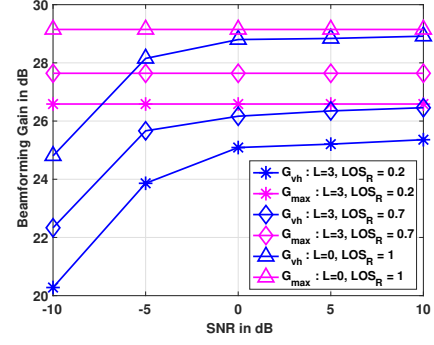
Figure 2: V-HiePM performance in channels with different power ratios between the dominant path and L = 3 scattered components.
