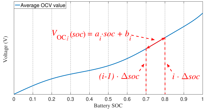
Figure 2: General shape of average OCV curve (example adapted from [24]).
