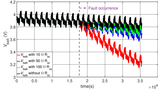
(a) V_{\text{batt}}
