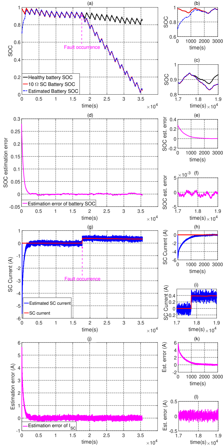
24 Figure 9: (a) SOC estimation result; (b) enlargement of the beginning; (c) dynamic estimation performance after fault occurrence; (d)/(e)/(f) estimation error corresponding to (a)/(b)/(c); (g) SC current estimation result; (h) enlargement of the beginning; (i) dynamic estimation performance after fault occurrence; (j)/(k)/(l) estimation error corresponding to (g)/(h)/(i).
