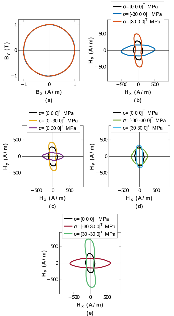
Fig. 8. Measured B - and H -loci for CW rotation of the field under 1 T induction level and several stress states. (a) B -loci under each case. (b) H -loci under zero and uniaxial stress along rolling direction. (c) H -loci under zero and uniaxial stress along transverse direction. (d) H -loci under zero and equibiaxial stress. (e) H -loci under zero and pure shear stress.
