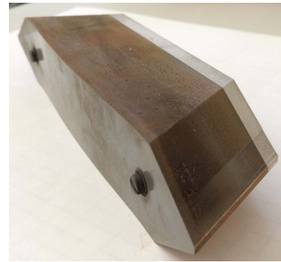
Fig. 3. Magnetizing yoke.
