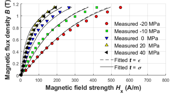
Fig. 1. Fitting of (1)-(2) to magnetization curves measured under uniaxial stresses parallel to the field.
