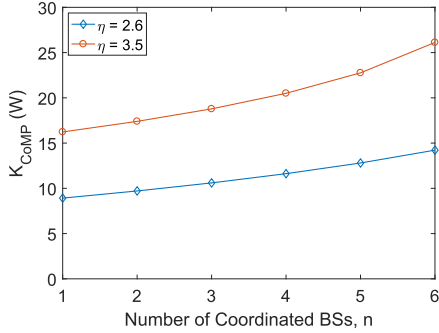
Fig. 11: K_{CoMP} vs the number of coordinated BSs n in a MCN
